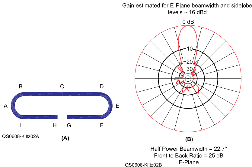
Figure 2 — At A, portion of a printout from VK5DJ's Yagi Calculator . At B, polar pattern for 24 element DL6WU Yagi at 1296 MHz.
