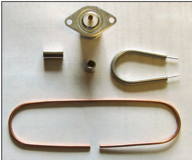
Figure 10 — Parts used to make folded dipole driven element.
