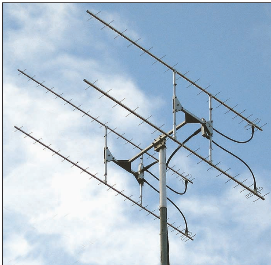
Figure 1 — Array of Yagi pairs for 23 and 33 cm on 6-foot booms.
